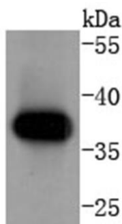
Fig. 1. Western blot analysis of Cyclin H on K562 cells lysates using anti-Cyclin H antibody at 1/1,000 dilution.
